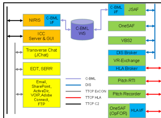
Figure 4: Architecture for UK CAGE IIIb Node.
